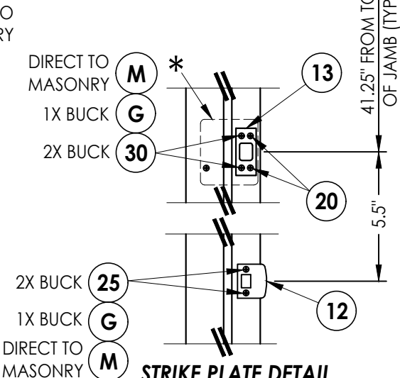
STRIKE PLATE DETAIL KWIKSET LOCKSET
